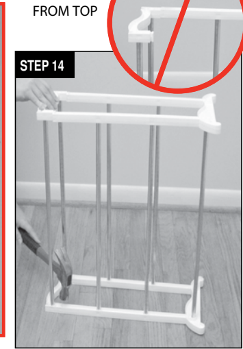
STEP 14: Tap connections together as shown, on a firm surface only.
