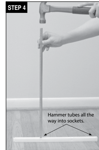
STEP 4: Assemble Uprights. Firmly hammer tubes into sockets.
