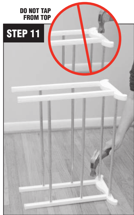
STEP 11: Tap connections together as shown, on a firm surface only.
