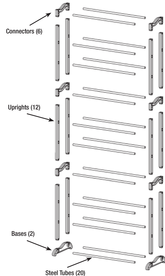
STEP 6: Repeat with remaining Uprights.
