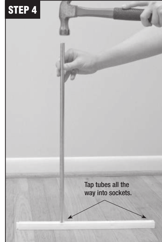
STEP 4: Assemble Uprights. Firmly tap tubes into sockets.
