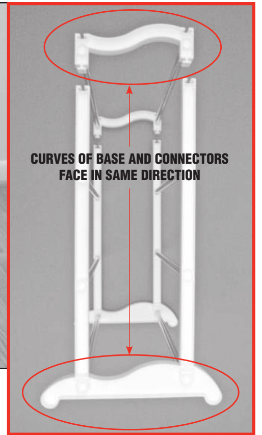
STEP 13: Add Connectors, align in same direction as Base as shown.
